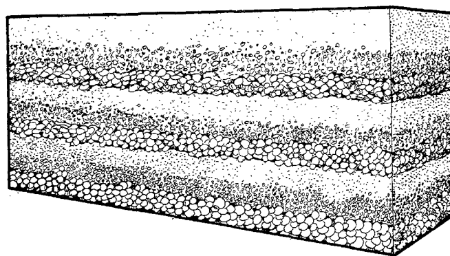
FIGURE 2. A block diagram showing a cross-section through three graded sedimentary beds. In each bed, the larger particles are at the bottom, and the smaller particles at the top.
